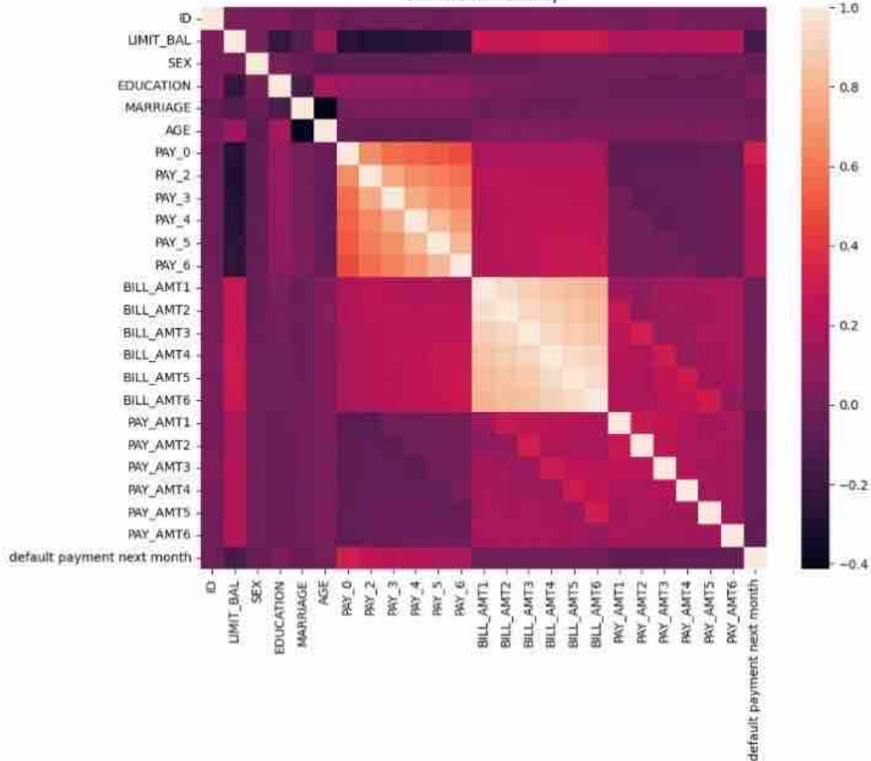
Correlation Heatmap
