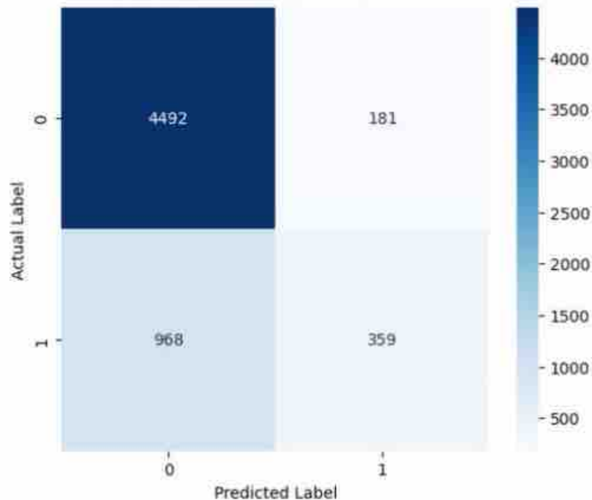
Confusion Matrix - SVM
